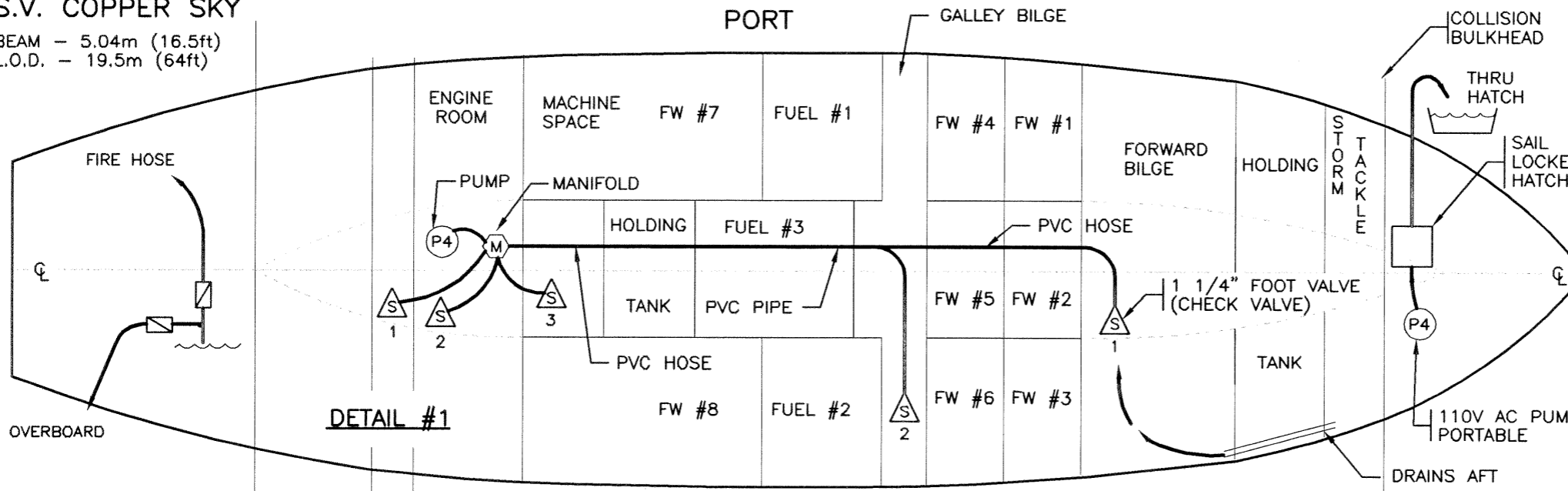
STARBOARD PLAN VIEW NTS
