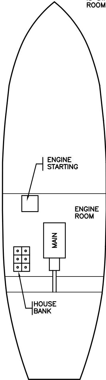
PLAN VIEW NTS
